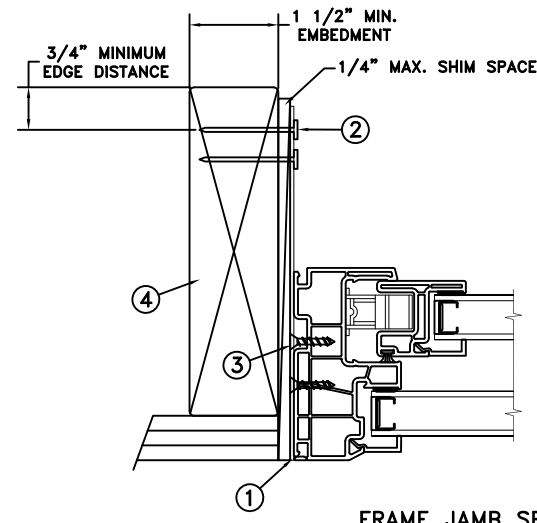
FRAME JAMB SECTION (TYP) HORIZONTAL SECTION
